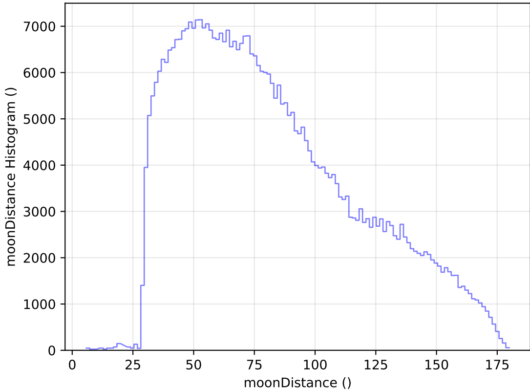
internal_u_expt30_nscale1.5v3.4_10yrs All sky z band: moonDistance Histogram
