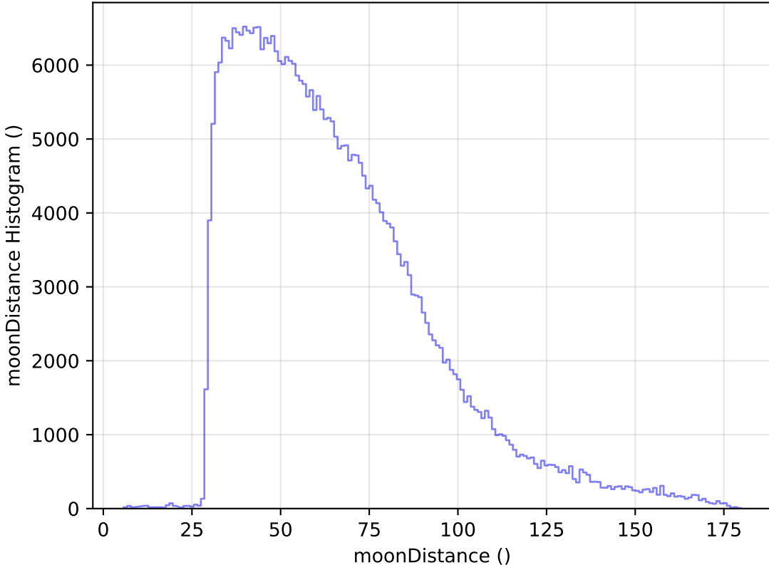
internal_u_expt30_nscale1.5v3.4_10yrs All sky y band: moonDistance Histogram
