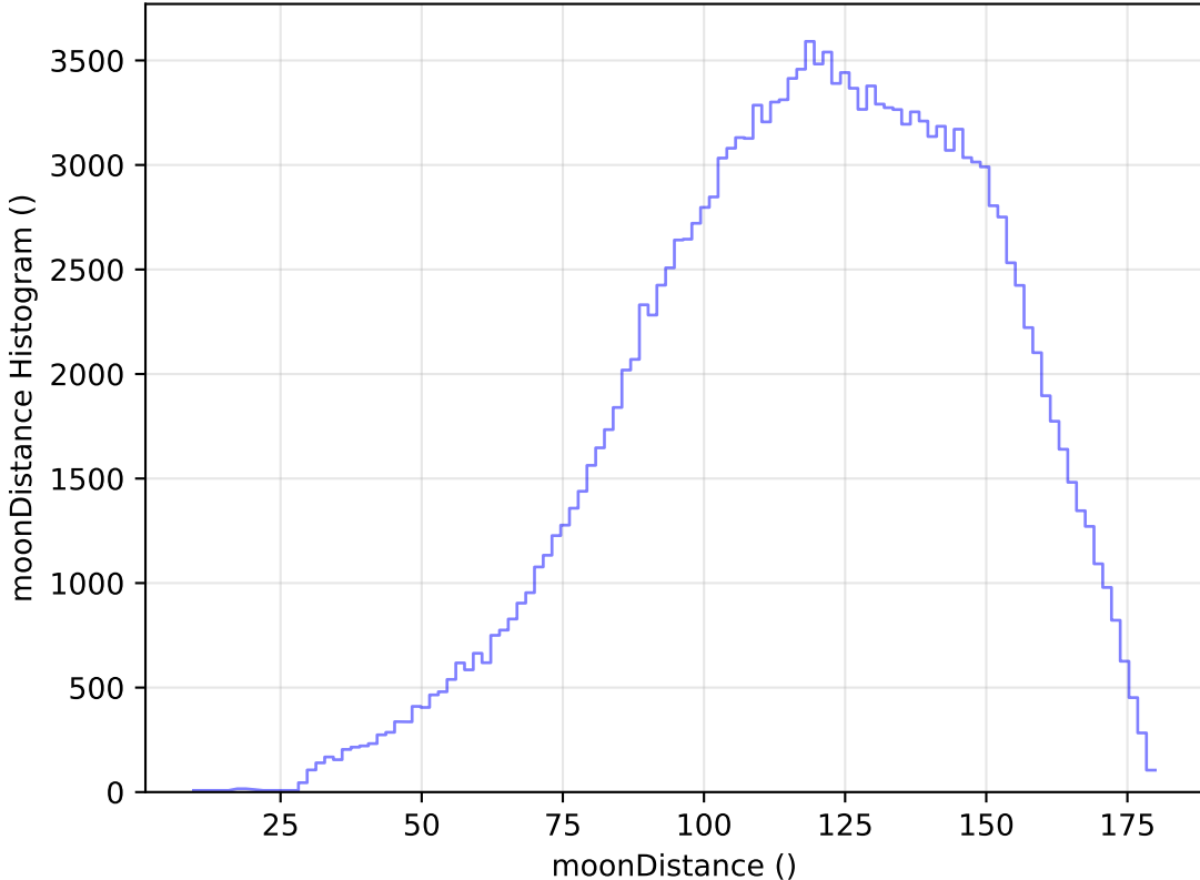
internal_u_expt30_nscale1.5v3.4_10yrs All sky u band: moonDistance Histogram
