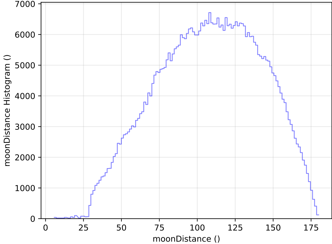
internal_u_expt30_nscale1.5v3.4_10yrs All sky r band: moonDistance Histogram
