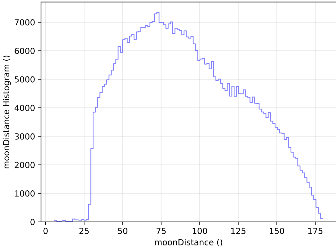
internal_u_expt30_nscale1.5v3.4_10yrs All sky i band: moonDistance Histogram
