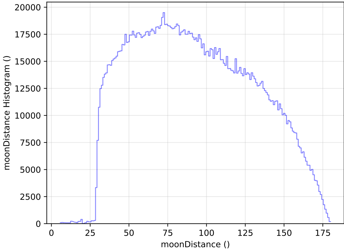
internal_u_expt30_nscale1.5v3.4_10yrs All sky all bands: moonDistance Histogram
