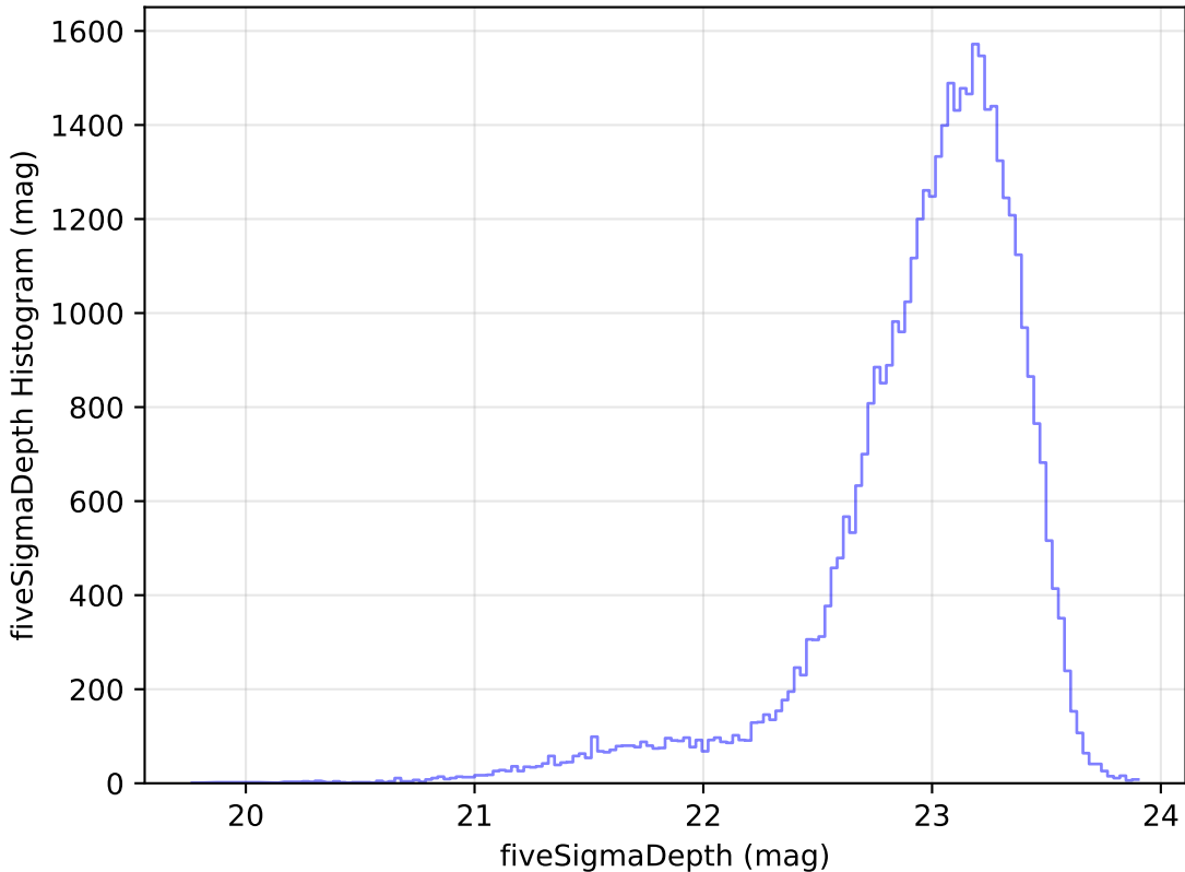
internal_u_expt30_nscale1.5v3.4_10yrs Yr 1 z band: fiveSigmaDepth Histogram
