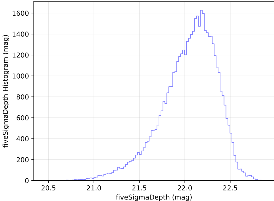
internal_u_expt30_nscale1.5v3.4_10yrs Yr 1 y band: fiveSigmaDepth Histogram
