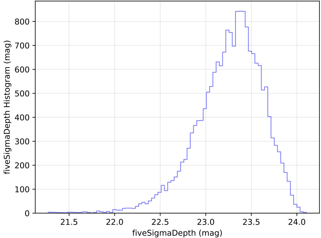
internal_u_expt30_nscale1.5v3.4_10yrs Yr 1 u band: fiveSigmaDepth Histogram
