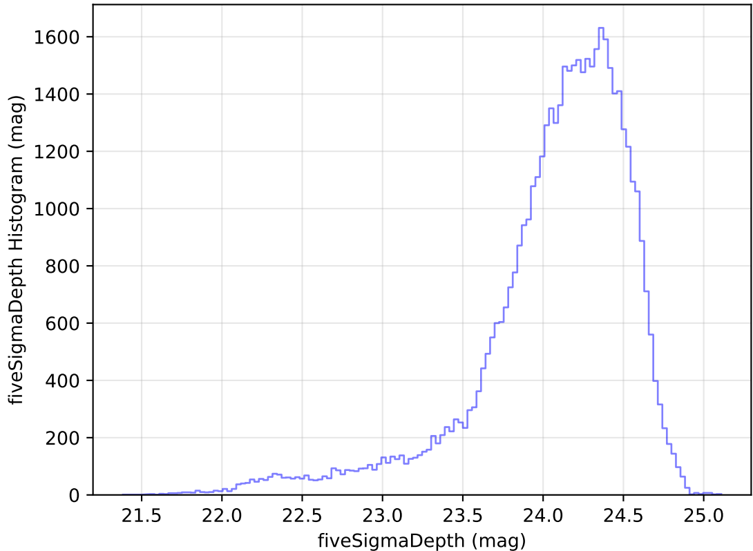
internal_u_expt30_nscale1.5v3.4_10yrs Yr 1 r band: fiveSigmaDepth Histogram
