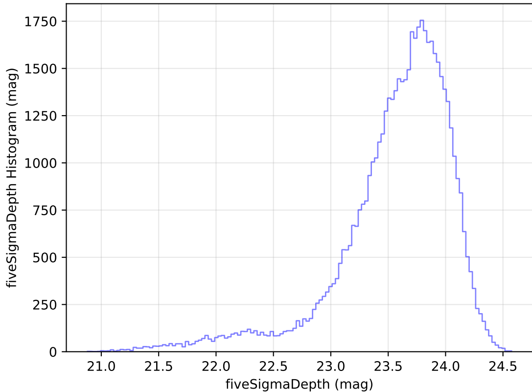
internal_u_expt30_nscale1.5v3.4_10yrs Yr 1 i band: fiveSigmaDepth Histogram
