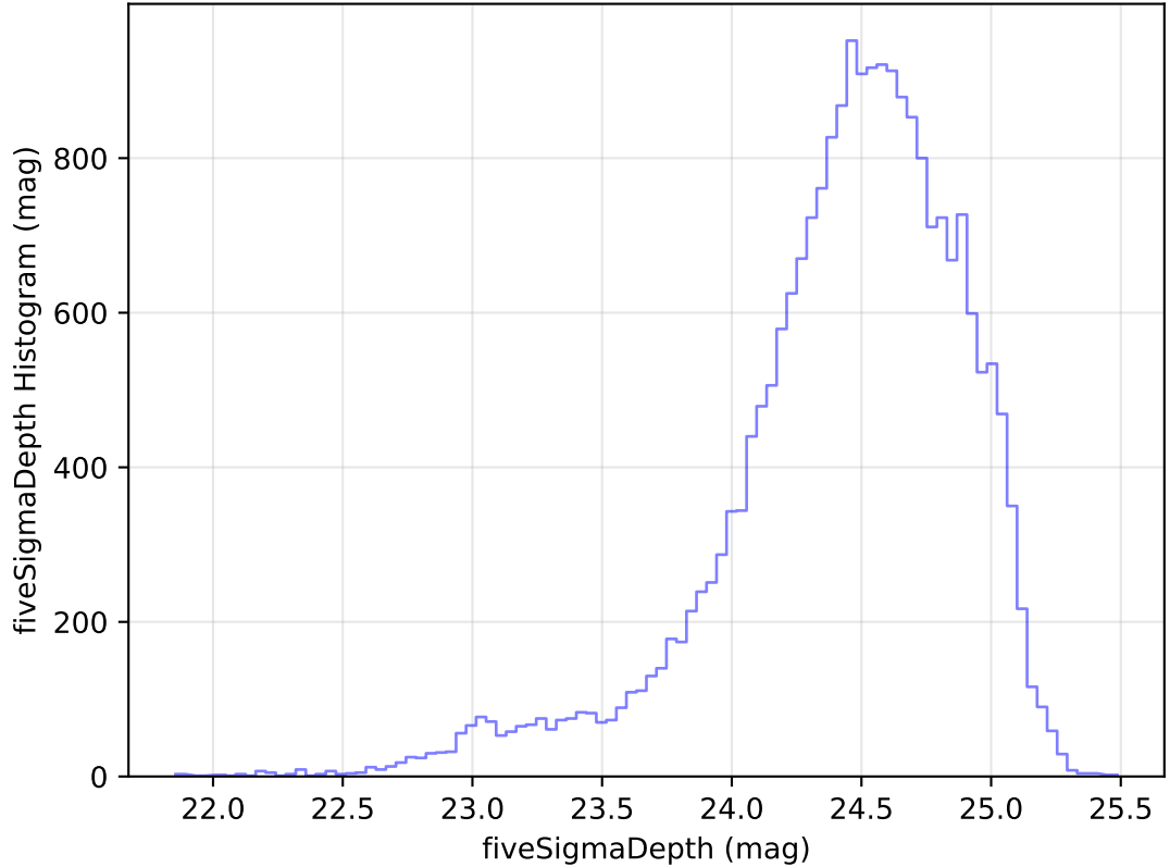
internal_u_expt30_nscale1.5v3.4_10yrs Yr 1 g band: fiveSigmaDepth Histogram
