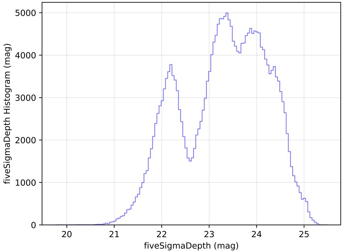
internal_u_expt30_nscale1.5v3.4_10yrs Yr 1 all bands: fiveSigmaDepth Histogram
