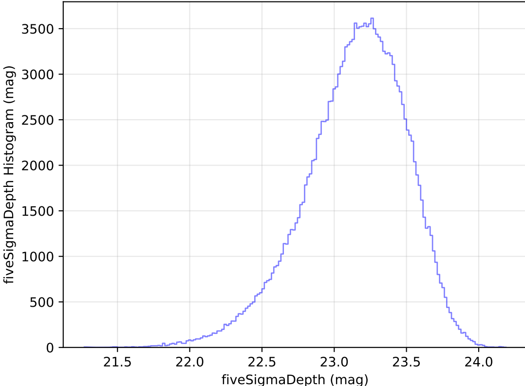
internal_u_expt30_nscale1.5v3.4_10yrs WFD u band: fiveSigmaDepth Histogram
