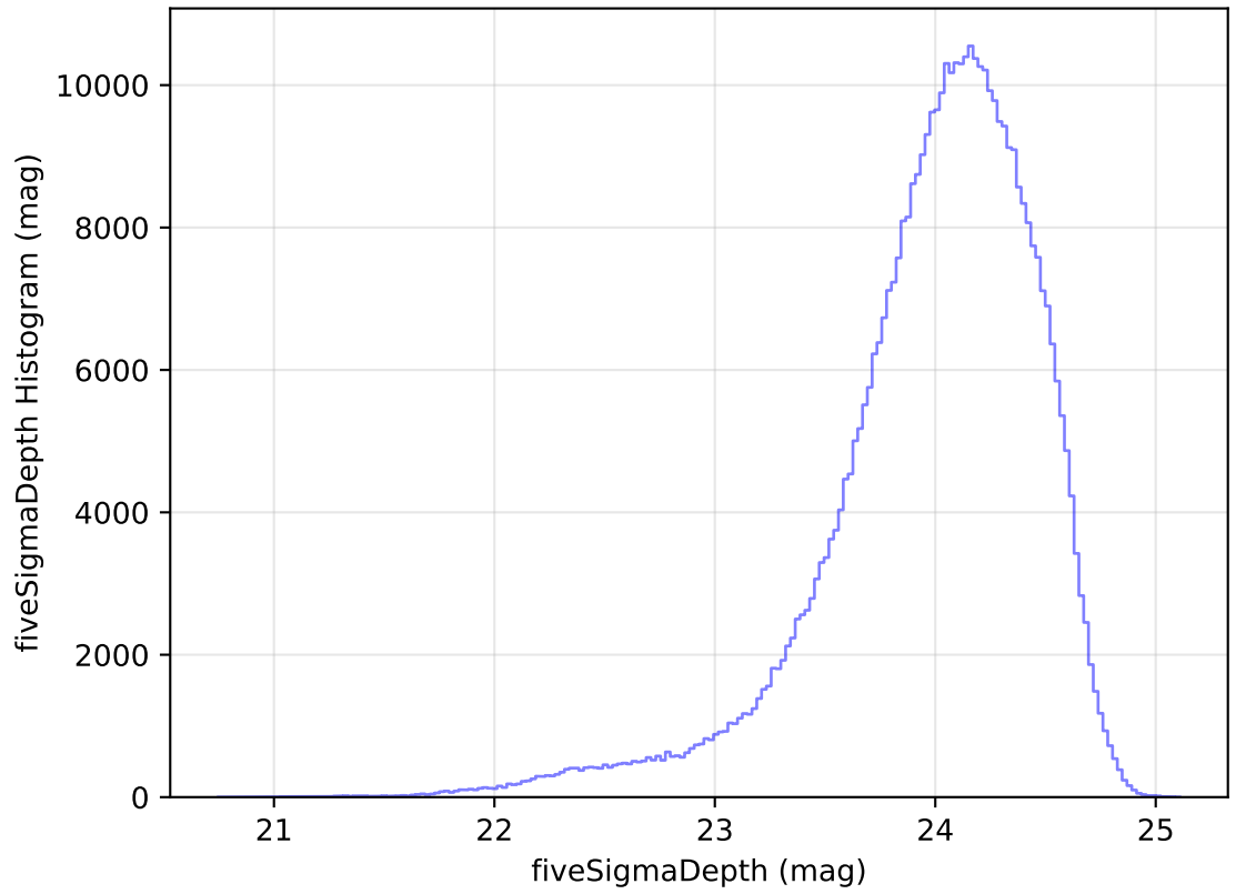
internal_u_expt30_nscale1.5v3.4_10yrs WFD r band: fiveSigmaDepth Histogram
