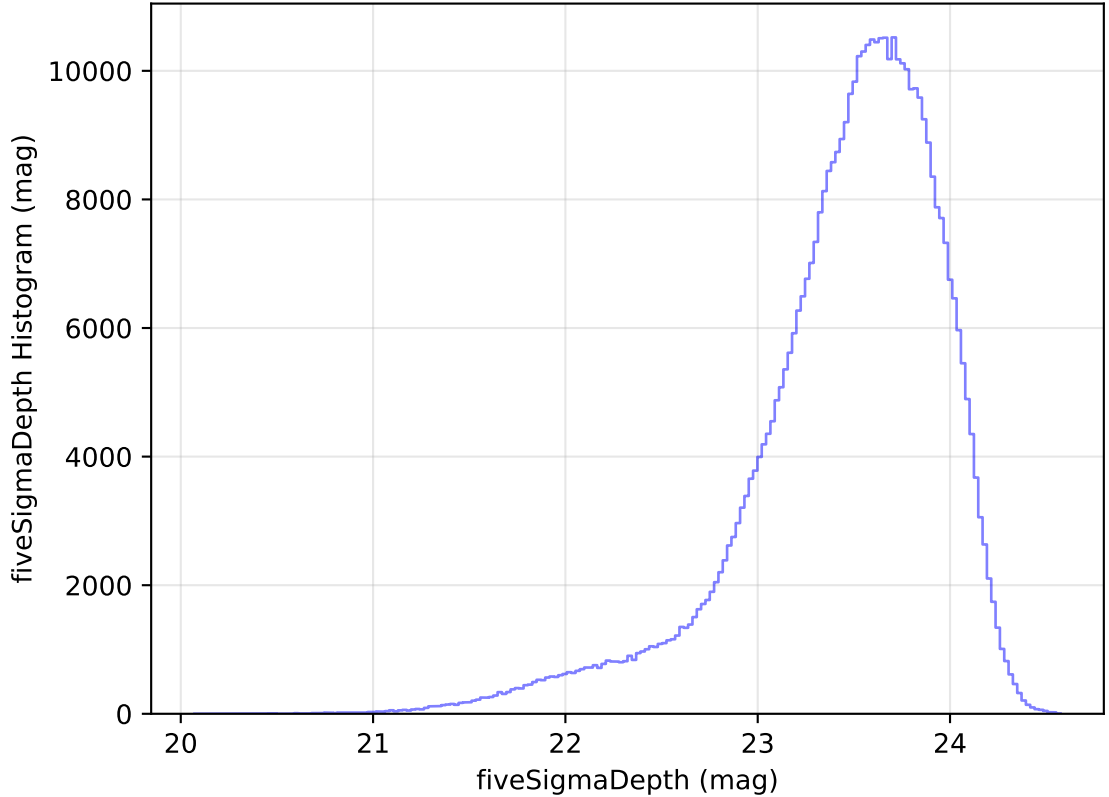
internal_u_expt30_nscale1.5v3.4_10yrs WFD i band: fiveSigmaDepth Histogram
