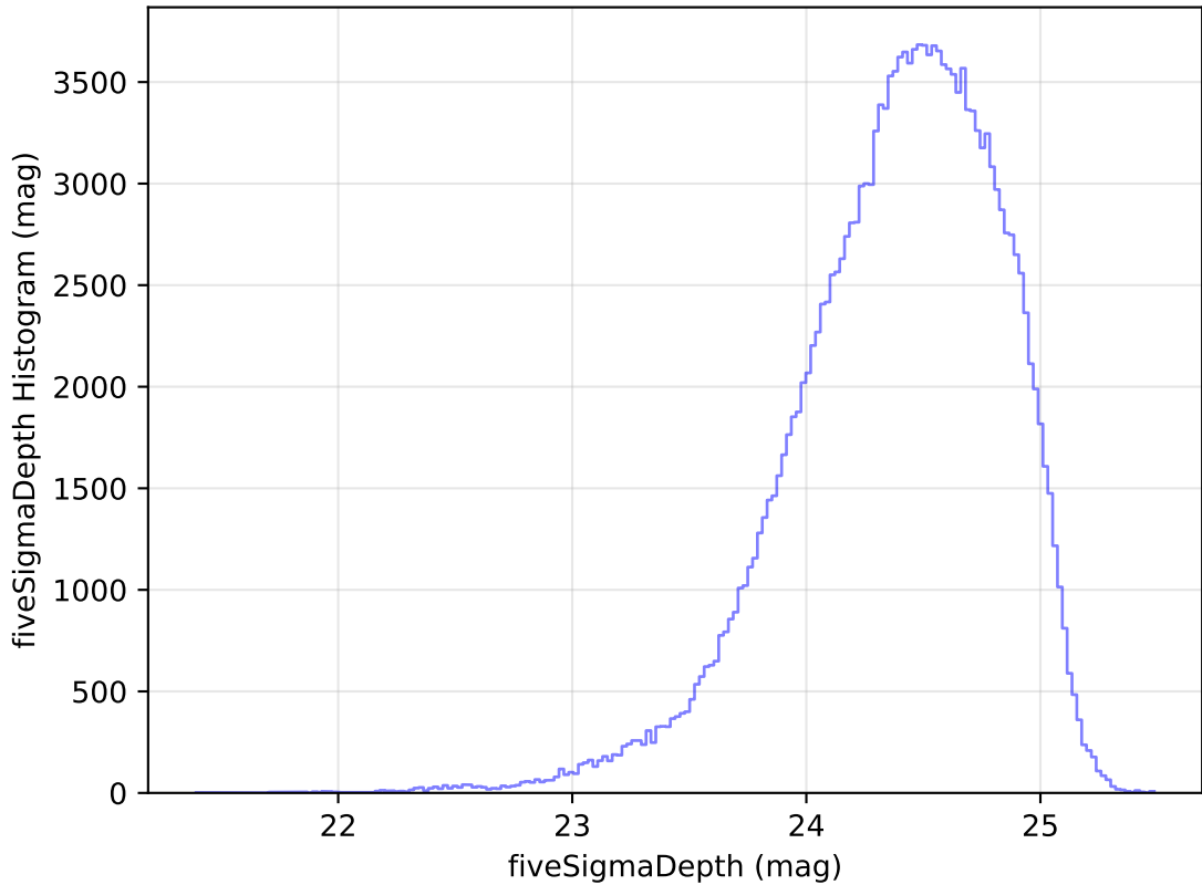
internal_u_expt30_nscale1.5v3.4_10yrs WFD g band: fiveSigmaDepth Histogram
