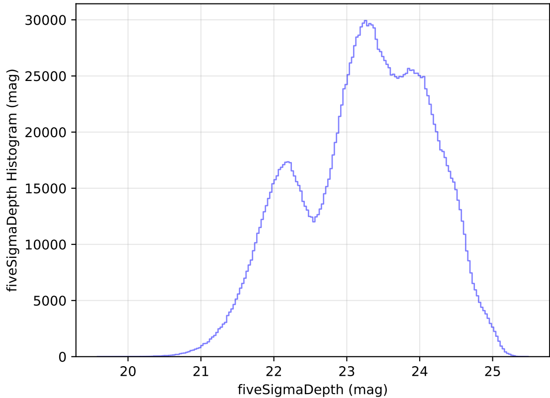
internal_u_expt30_nscale1.5v3.4_10yrs WFD all bands: fiveSigmaDepth Histogram
