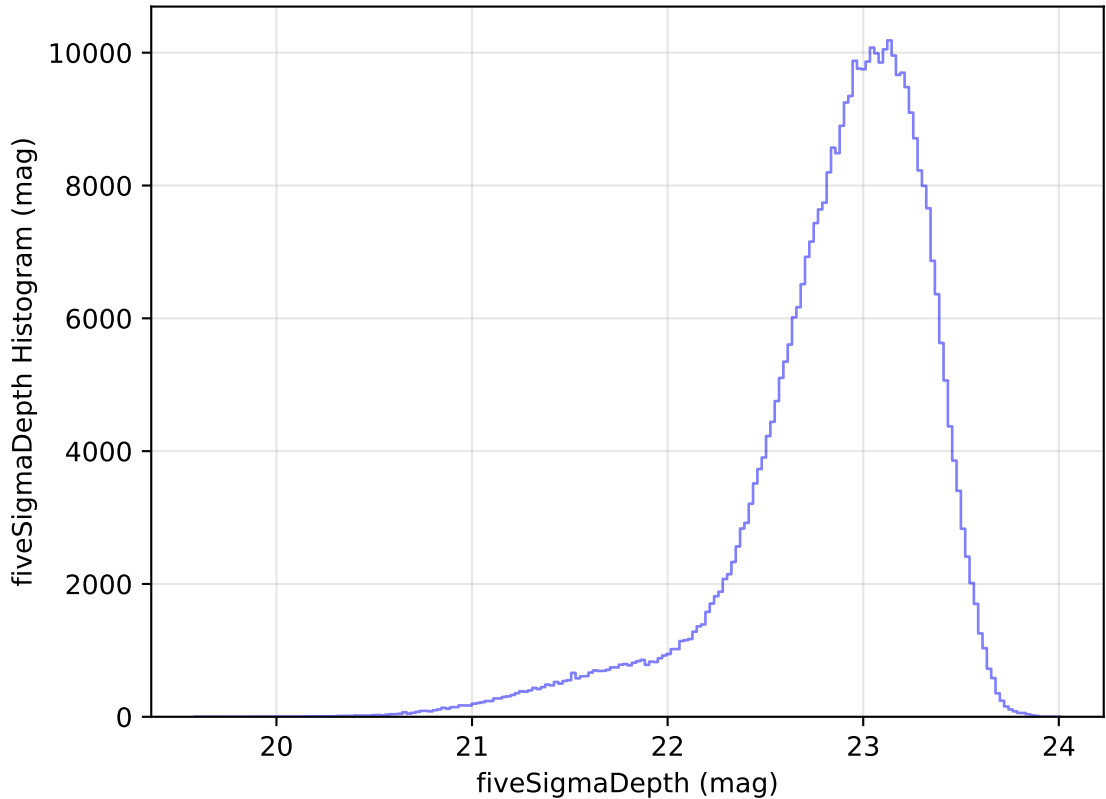
internal_u_expt30_nscale1.5v3.4_10yrs All sky z band: fiveSigmaDepth Histogram
