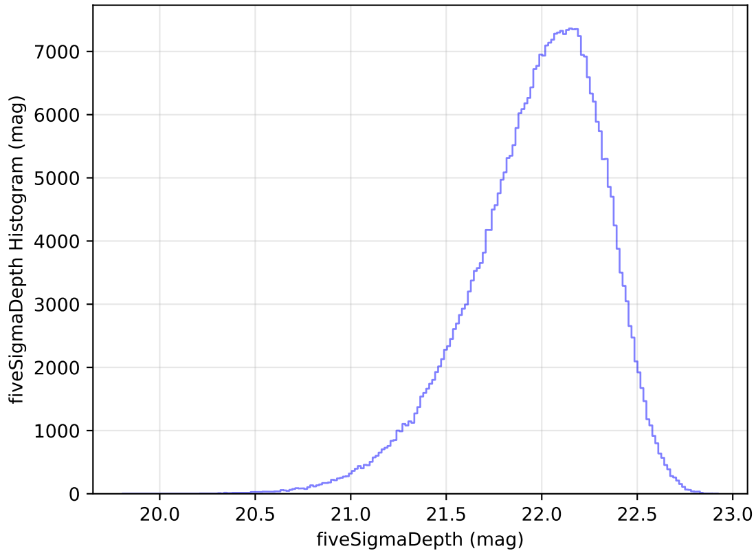
internal_u_expt30_nscale1.5v3.4_10yrs All sky y band: fiveSigmaDepth Histogram
