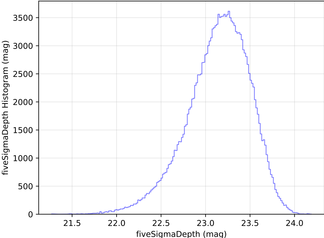
internal_u_expt30_nscale1.5v3.4_10yrs All sky u band: fiveSigmaDepth Histogram
