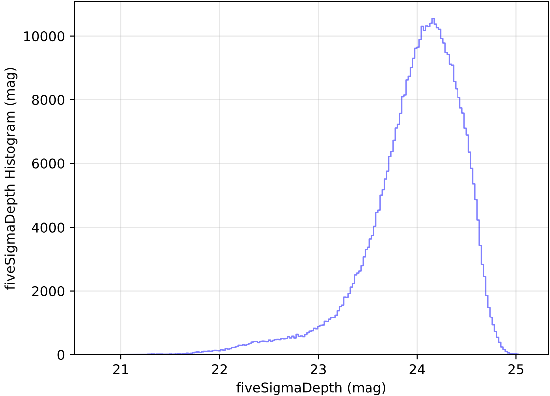
internal_u_expt30_nscale1.5v3.4_10yrs All sky r band: fiveSigmaDepth Histogram
