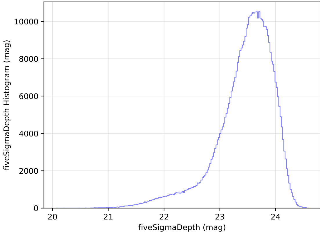
internal_u_expt30_nscale1.5v3.4_10yrs All sky i band: fiveSigmaDepth Histogram
