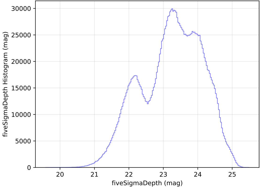
internal_u_expt30_nscale1.5v3.4_10yrs All sky all bands: fiveSigmaDepth Histogram
