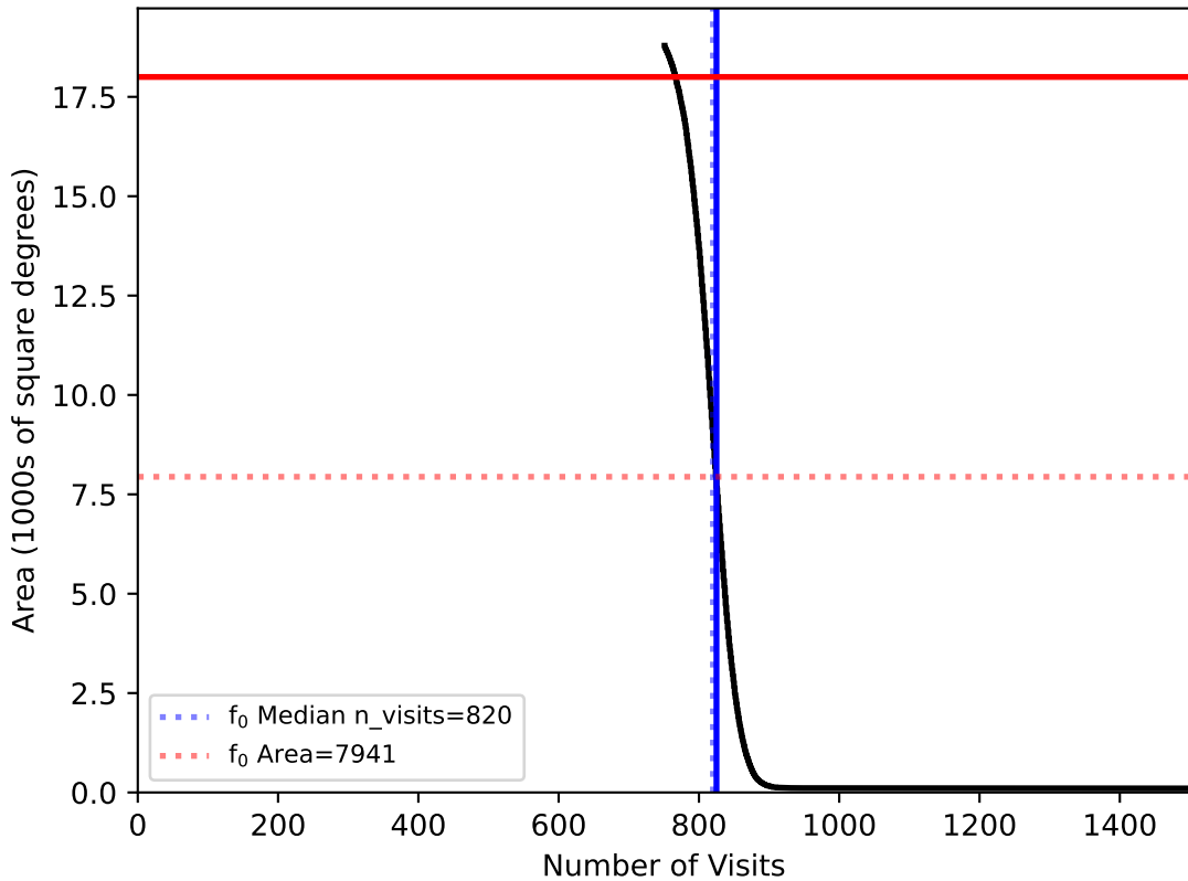
internal_u_expt30_nscale1.5v3.4_10yrs WFD: f0
