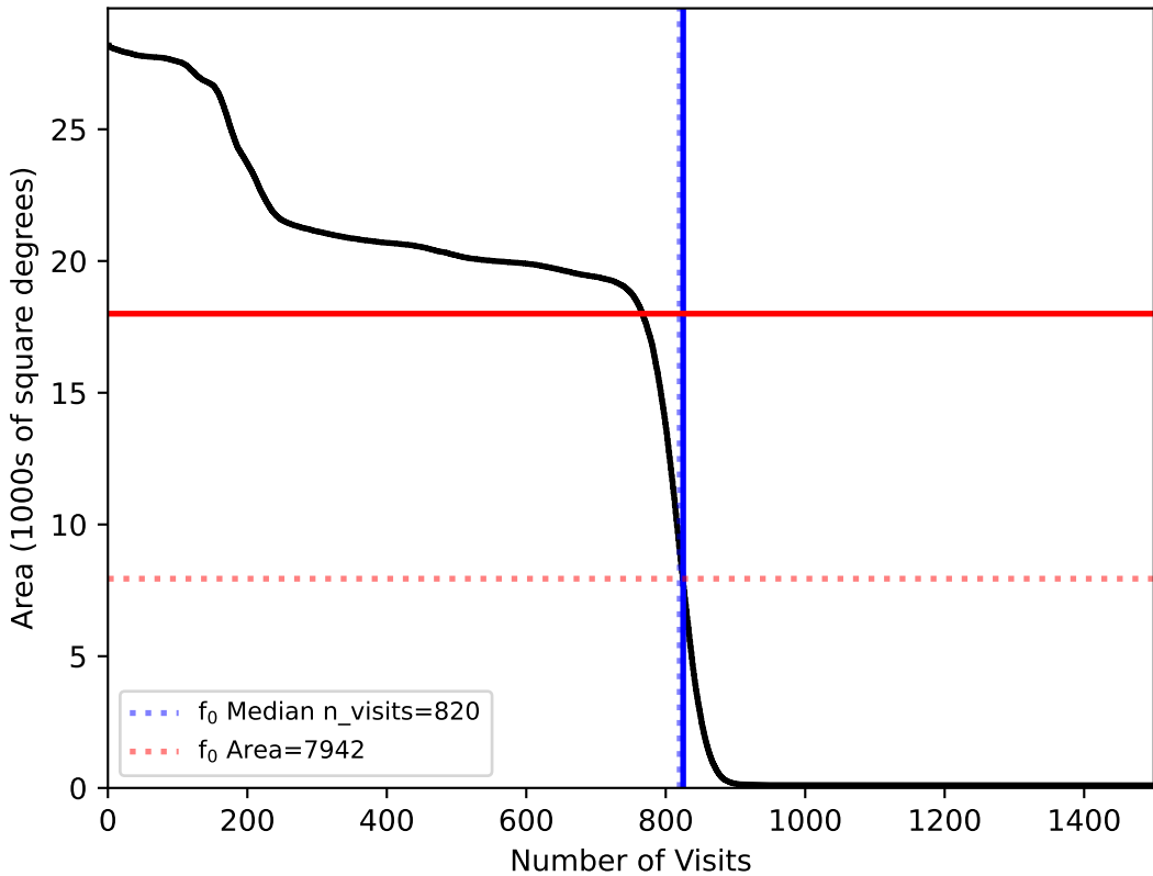
internal_u_expt30_nscale1.5v3.4_10yrs All sky: f0
