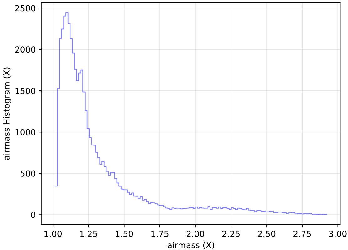
internal_u_expt30_nscale1.5v3.4_10yrs Yr 1 z band: airmass Histogram
