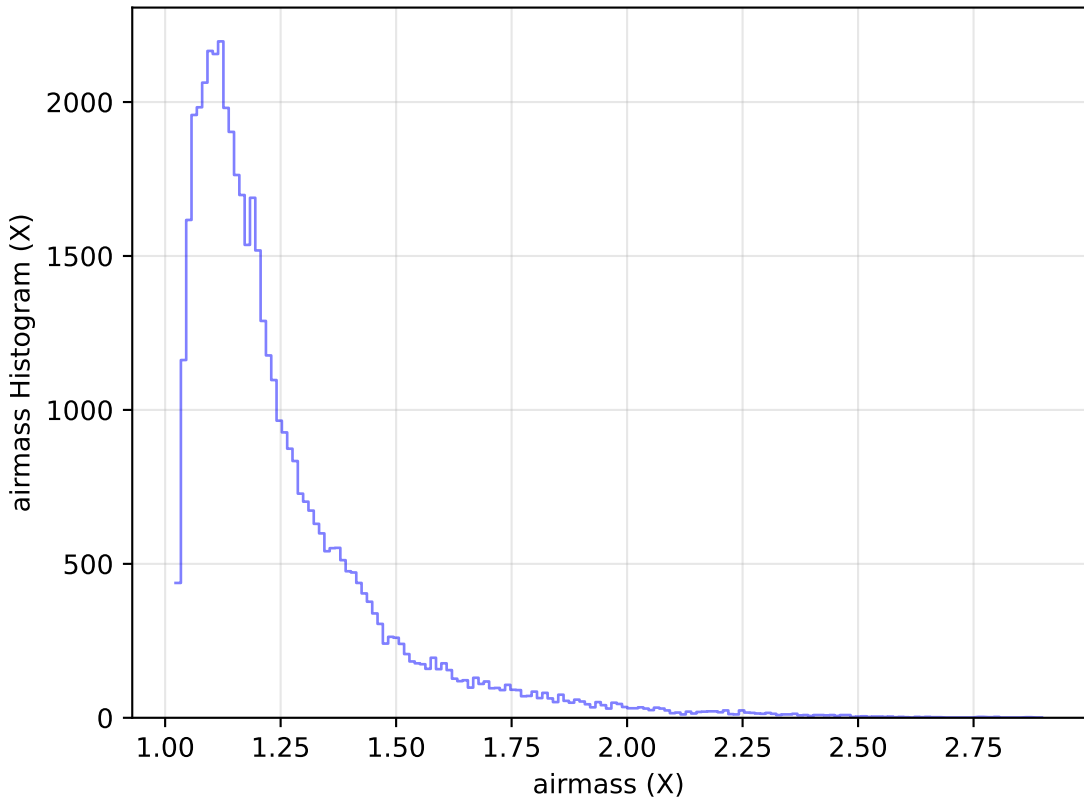
internal_u_expt30_nscale1.5v3.4_10yrs Yr 1 y band: airmass Histogram
