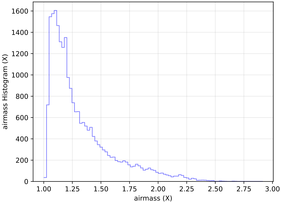
internal_u_expt30_nscale1.5v3.4_10yrs Yr 1 g band: airmass Histogram
