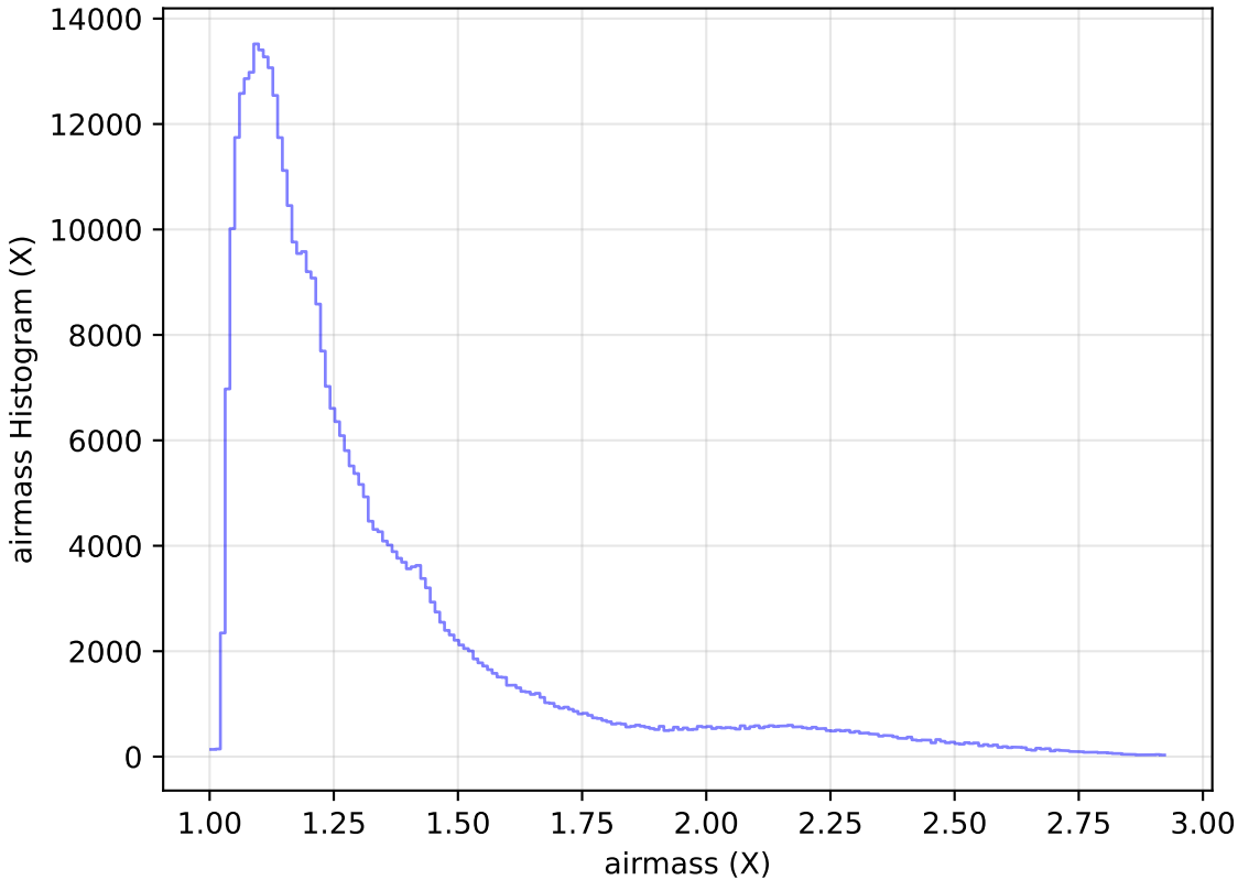
internal_u_expt30_nscale1.5v3.4_10yrs WFD z band: airmass Histogram
