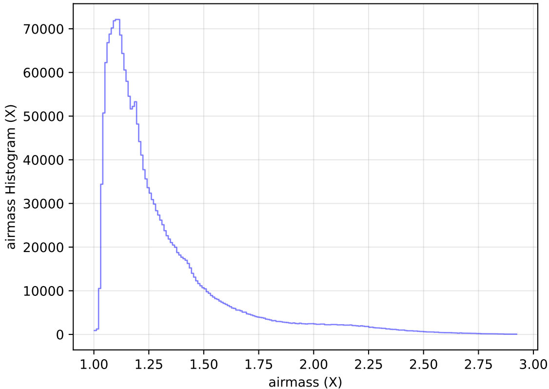
internal_u_expt30_nscale1.5v3.4_10yrs WFD all bands: airmass Histogram
