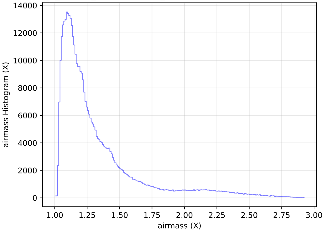
internal_u_expt30_nscale1.5v3.4_10yrs All sky z band: airmass Histogram
