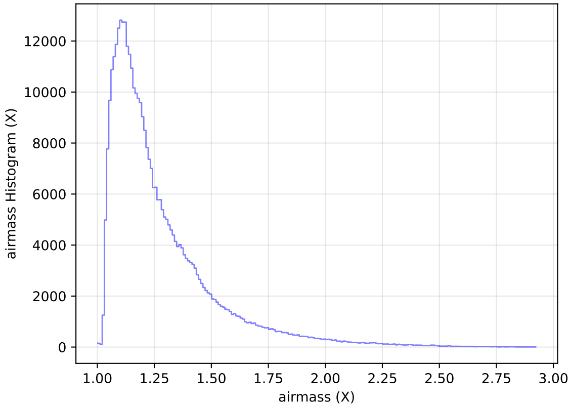
internal_u_expt30_nscale1.5v3.4_10yrs All sky y band: airmass Histogram
