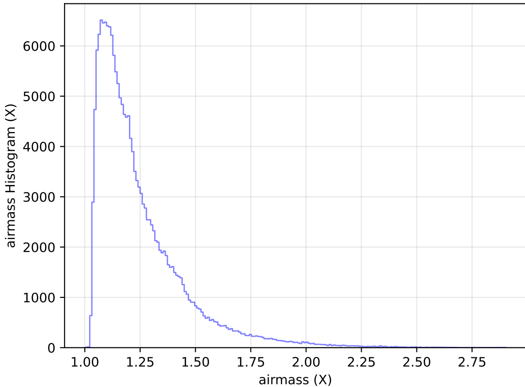
internal_u_expt30_nscale1.5v3.4_10yrs All sky u band: airmass Histogram
