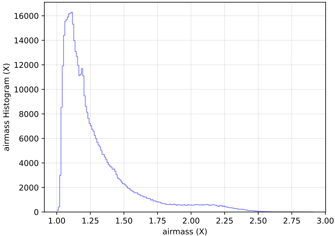
internal_u_expt30_nscale1.5v3.4_10yrs All sky r band: airmass Histogram
