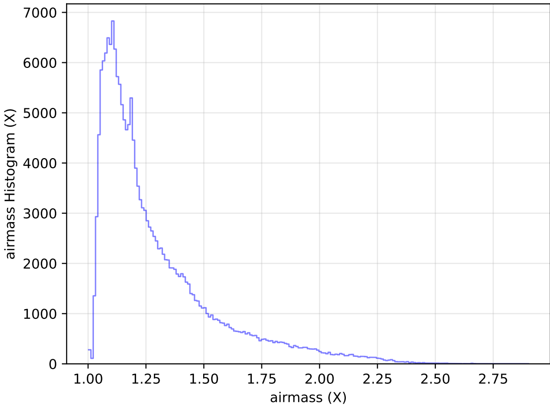
internal_u_expt30_nscale1.5v3.4_10yrs All sky g band: airmass Histogram
