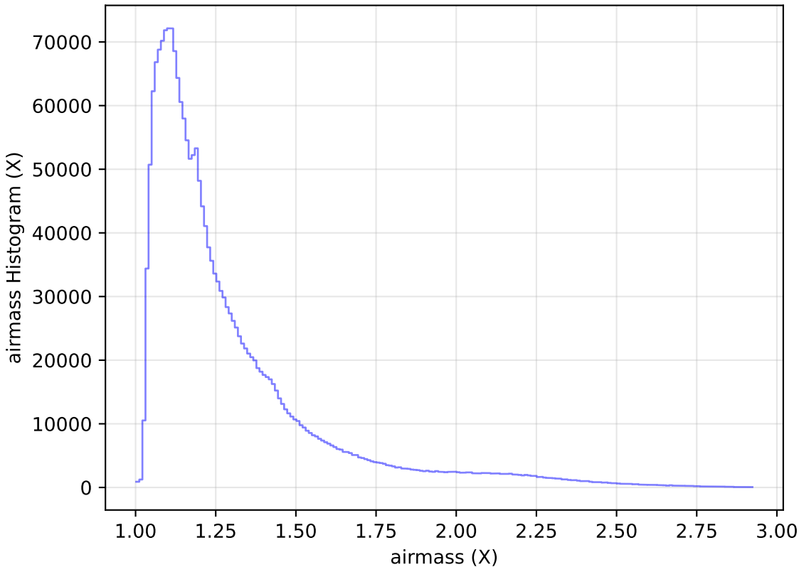
internal_u_expt30_nscale1.5v3.4_10yrs All sky all bands: airmass Histogram
