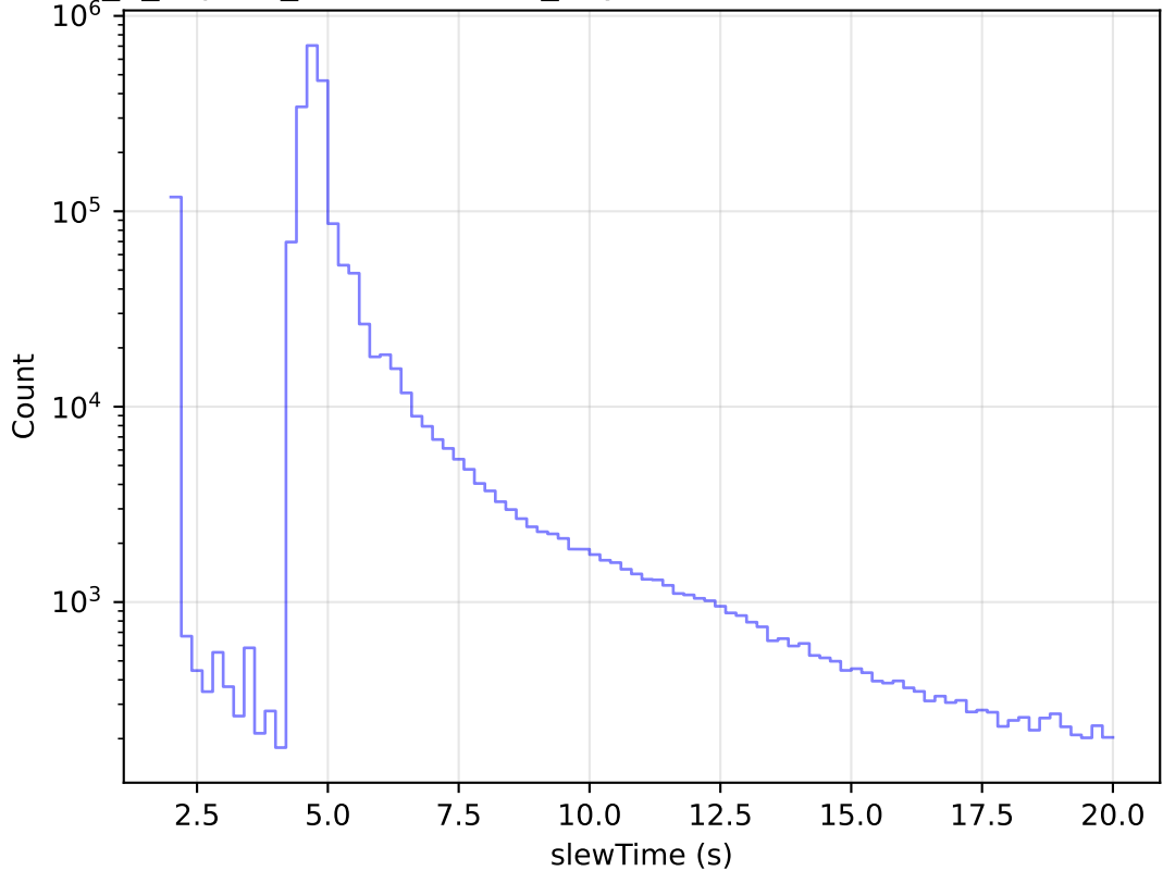
internal_u_expt30_nscale1.5v3.4_10yrs All visits: Zoom Slew Time Histogram
