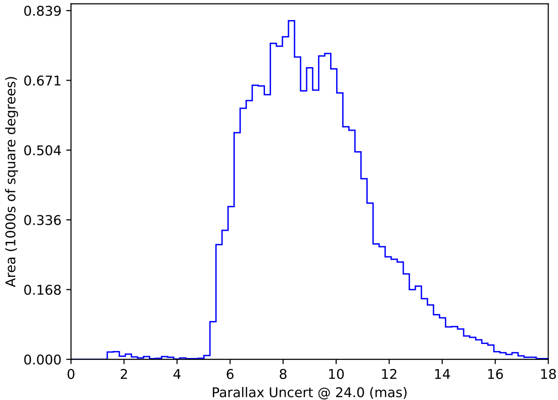
internal_u_expt30_nscale1.5v3.4_10yrs WFD: Parallax Uncert @ 24.0
