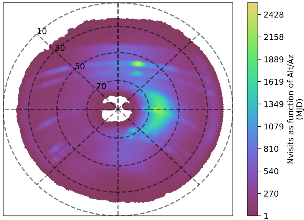
internal_u_expt30_nscale1.5v3.4_10yrs z band: Nvisits as function of Alt/Az
