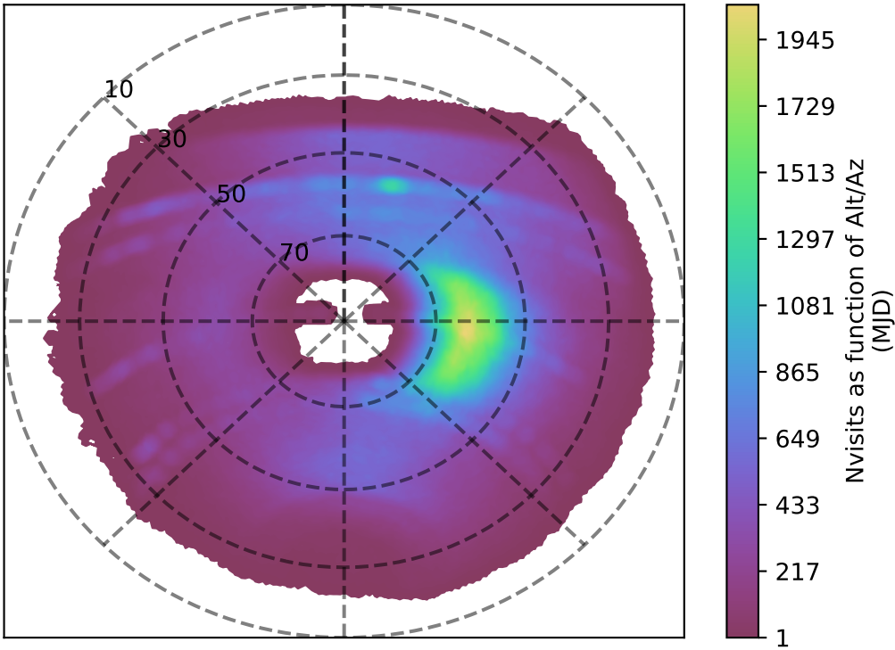
internal_u_expt30_nscale1.5v3.4_10yrs y band: Nvisits as function of Alt/Az
