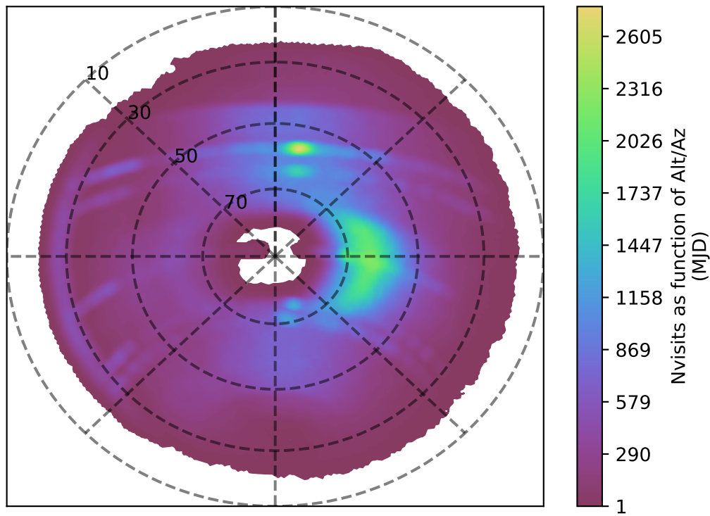
internal_u_expt30_nscale1.5v3.4_10yrs r band: Nvisits as function of Alt/Az
