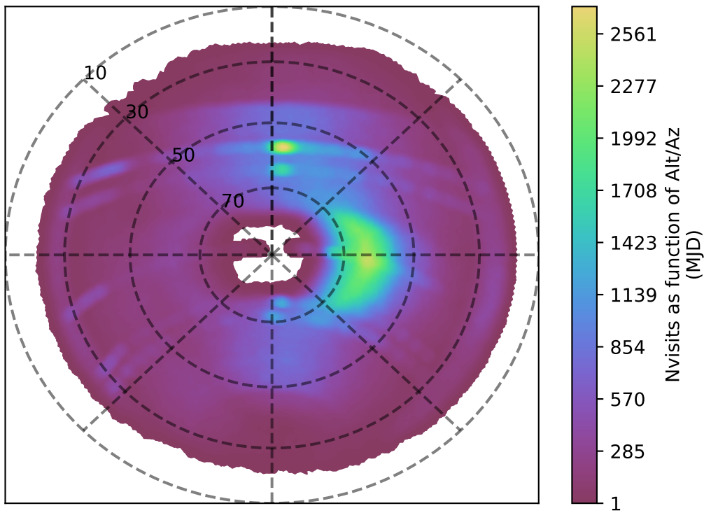
internal_u_expt30_nscale1.5v3.4_10yrs i band: Nvisits as function of Alt/Az
