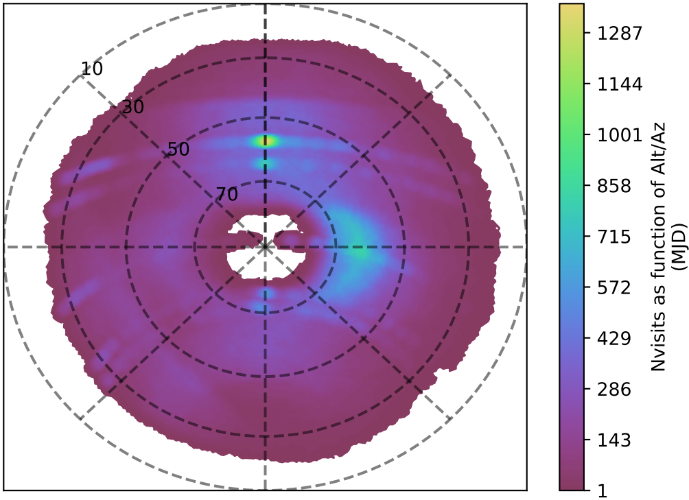
internal_u_expt30_nscale1.5v3.4_10yrs g band: Nvisits as function of Alt/Az
