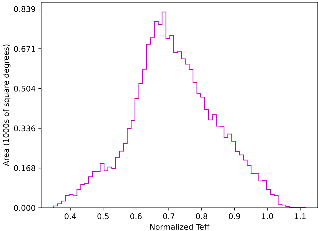
internal_u_expt30_nscale1.5v3.4_10yrs WFD z band: Normalized Teff
