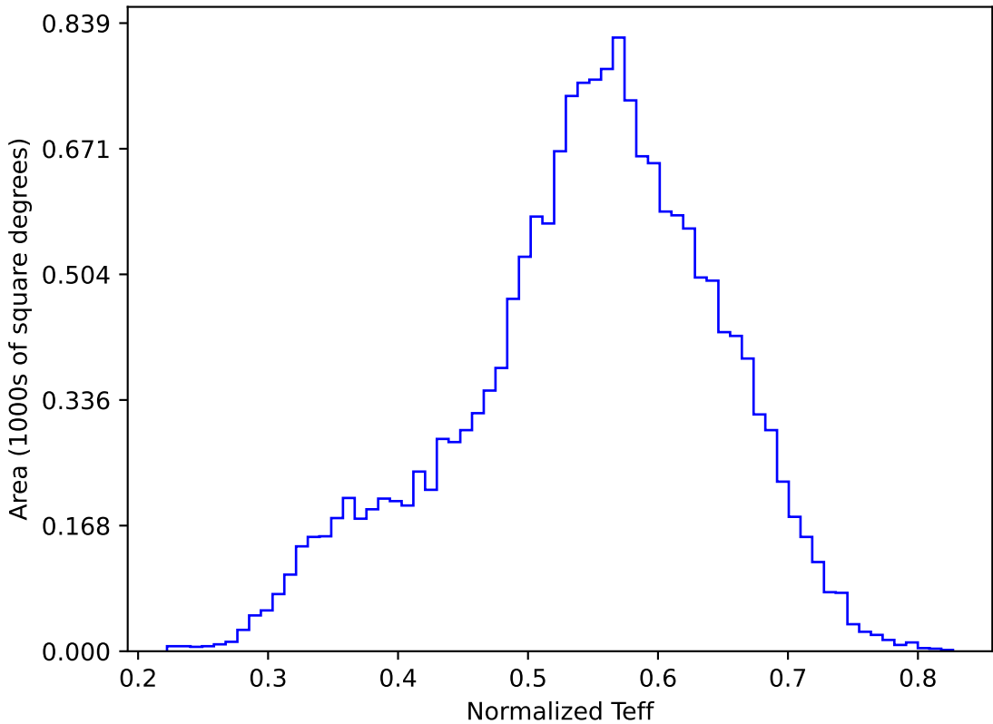
internal_u_expt30_nscale1.5v3.4_10yrs WFD y band: Normalized Teff
