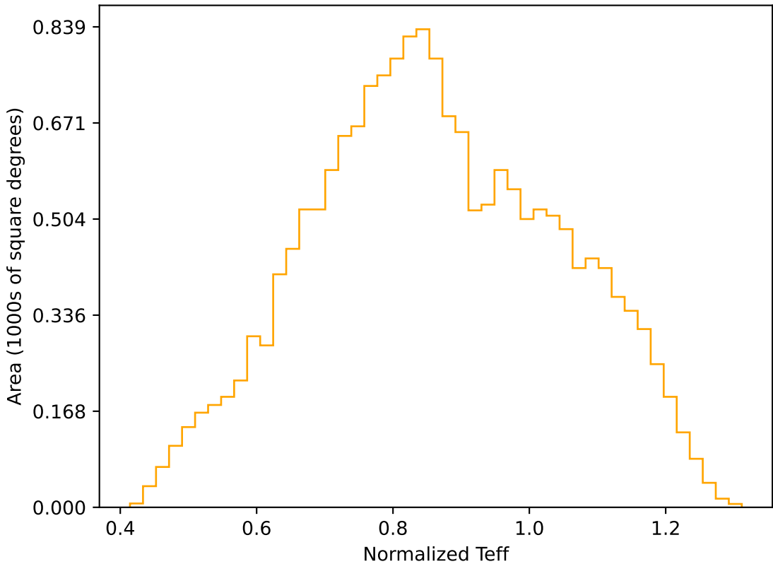
internal_u_expt30_nscale1.5v3.4_10yrs WFD r band: Normalized Teff
