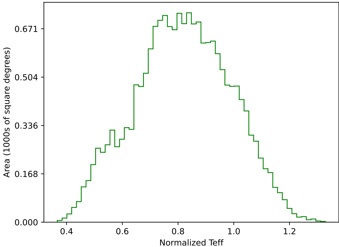
internal_u_expt30_nscale1.5v3.4_10yrs WFD g band: Normalized Teff
