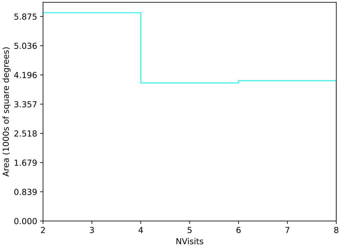
internal_u_expt30_nscale1.5v3.4_10yrs Yr 3-4 u band: NVisits
