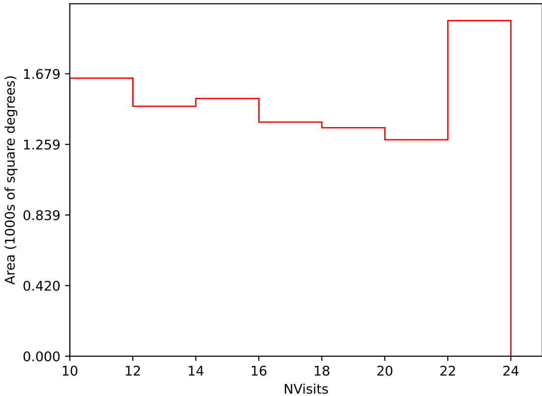
internal_u_expt30_nscale1.5v3.4_10yrs Yr 3-4 i band: NVisits
